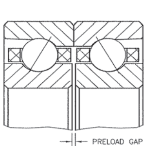
B-TYPE DUPLEX BACK-TO-BACK (DB)
